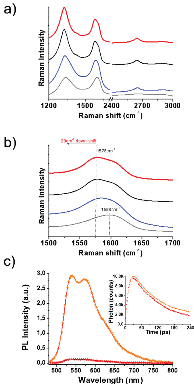
Fig. 2 (a) Full Raman spectra ( \lambda_{\text{exc}} 633 nm) and (b) expansion of the G-band of 1/S-G (red), GO (grey), SG (black) and 1/S-G (blue). (c) Photoluminescence spectra ( \lambda_{\text{exc}} 441 nm) of 1 (orange) and 1/S-G (red) obtained in benzonitrile. Inset: Photoluminescence lifetime decay graphs.
