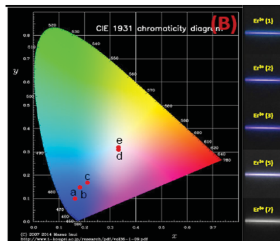
Fig. 9 (A) UCL spectra (B) corresponding 'Commission Internationale de l'Eclairage' (CIE) and digital images of CSS UCNP structures. a, b, c, d and e in the CIE diagram indicate the corresponding UCNP structures, having \text{Er}^{3+} concentrations 1, 2, 3, 5 and 7 mol%, respectively, in the outermost shell. Digital images are taken using an 808 nm laser, 10 \text{ W cm}^{-2} (without using any filter).
