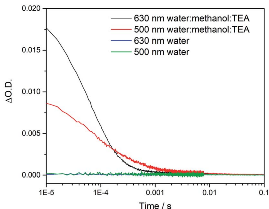
Fig. 6 Kinetic traces recorded at the wavelengths indicated for cLaP1 in either water alone or a \text{H}_2\text{O}/\text{TEA}/\text{MeOH} mixture under a nitrogen atmosphere following excitation with a 355 nm (6 ns, 400 \mu\text{J cm}^{-2} , 0.33 Hz) laser.
