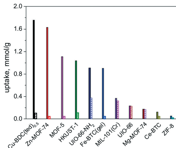
Fig. 1 \text{H}_2\text{S} uptake on different MOFs at 298 K under 1 atm ( \text{H}_2\text{S} , 1 kPa; filled column: fresh MOF adsorbents; striped column: ref refreshed adsorbents). Reproduced with permission from ref. 38.
