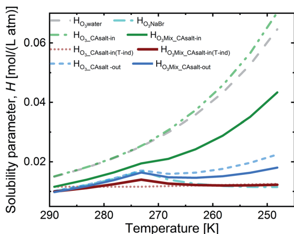
Fig. 4 Calculated ozone solubility in solution fractions and in the mixture (by the volume mixing rule). H_{O_3i} is Henry's law O_3 solubility in solution (i). Grey dashed line: H_{O_3water} ; cyan dash-dot line: H_{O_3NaBr} ; green dash-dot-dot line: H_{O_3-CA_{salt-in}} , salting-in effect with T dependence of H_{O_3water} ; red dotted line: H_{O_3-CA_{salt-in}(T-ind)} , salting-in effect without T -dependence; blue dashed line: H_{O_3-CA_{salt-out}} , salting-out effect with T dependence of H_{O_3water} ; solid green line: H_{O_3-Mix_{CA_{salt-in}}} with H_{O_3-CA_{salt-in}} ; solid red line: H_{O_3Mix_{CA_{salt-in}(T-ind)}} with H_{O_3-CA_{salt-in}(T-ind)} ; solid blue line: H_{O_3Mix_{CA_{salt-out}}} with H_{O_3-CA_{salt-out}} ; all H_{O_3Mix} contain volume ratio combinations of the H_{O_3-CA} scenarios and H_{O_3NaBr} surface reaction.
