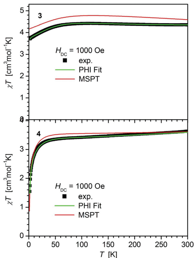
Fig. 3 Temperature dependence of \chi T for 3 and 4. Solid green lines represent the results of the simultaneous fittings with the temperature dependent magnetization (Table 3, Fig. S12†) according to a spin Hamiltonian (eqn (S1)†) by the PHI program. 21 Red lines represent the results of the quantum chemical calculations (MS-CAS(12,13)PT2) (see also Fig. S24†).
