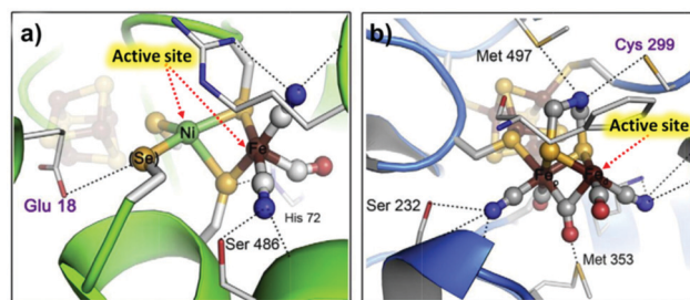
Fig. 13 X-ray structures of (a) NiFe cluster of [\text{NiFe}(\text{Ser})] -hydrogenases; (b) 2Fe sub-cluster of the [\text{FeFe}] -hydrogenase H cluster. Adapted with permission from ref. 314. Copyright 2015 Elsevier.
