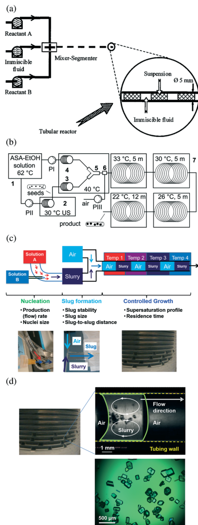
Fig. 4 (a) Segmented-flow crystallizer for reaction precipitation, with segments generated by a segmenter. 17 Reprinted from ref. 17, with permission from Wiley. (b) Segmented/slug-flow crystallizer for cooling crystallization, 29 with slugs generated by air inlet. A sonication bath is used for generating seeds, which are then mixed with saturated solution at a high temperature before slug formation. Reprinted with permission from ref. 29, Copyright 2012 American Chemical Society. (c) A slug-flow continuous crystallizer design with decoupled sub-processes (crystal nucleation, slug formation, and crystal growth). Each sub-process has the photos of corresponding key equipment shown in the bottom part of the figure, and the key design considerations listed then elaborated in section 2. For example, stable slugs in the slug-formation sub-process refers to slugs that do not combine nor separate after formation, which affects the recirculation mixing pattern within slugs and the control of crystal size distribution inside the slugs. The supersaturation could be generated from cooling, antisolvent, and/or reaction crystallization. Although the nucleation method shown in the figure uses micromixers, other methods can be used (e.g., ultrasonication in Fig. 6). Modified with permission from ref. 10, Copyright 2014 American Chemical Society. (d) (upper right) In-line video snapshot of a representative liquid slug (boundaries in green, internal fluid motion in white arrows), separated by two air slugs inside a tube (inner walls in yellow). 134 The whole crystallizer is composed of a series of identical liquid slugs where crystallization occurs. Modified with permission from ref. 10, Copyright 2014 American Chemical Society. (Bottom) Off-line microscope image of product crystals from a representative slug. Experimental conditions are detailed in ref. 10.
