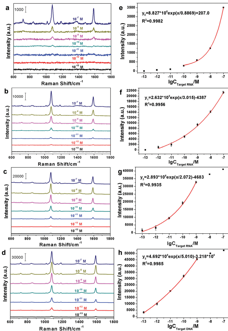
Fig. 4 SERS spectra corresponding to the different concentrations of miRNA-21 by (a) initial detection, (b) first order amplification detection, (c) second order amplification detection and (d) third order amplification detection; (e–h) the dose–response curves corresponding to (a–d), respectively.
