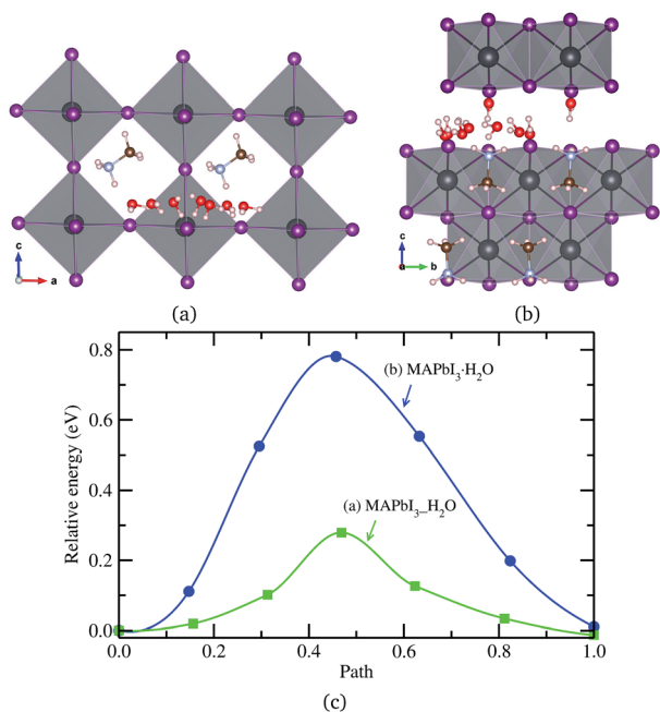
Fig. 6 \text{H}_2\text{O} molecule migrations in (a) water intercalated phase \text{MAPbI}_3 \cdot \text{H}_2\text{O} and (b) monohydrated phase \text{MAPbI}_3 \cdot \text{H}_2\text{O} , and (c) corresponding activation energy profile.
