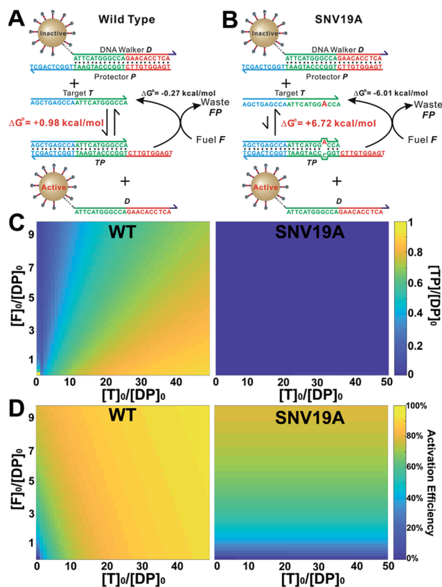
Fig. 1 Sequence-level tuning of the 3D DNA nanomachine (3DDN) for discriminating SNVs. (A and B) The toehold-exchange motif (DP) of the 3DDN consists of a DNA walker (D) and pre-hybridized protecting strand (P). This motif can react with an intended target (T) to release D for the subsequent stochastic walking along the AuNP track. Under the optimal sequence design ( f = 10 nt, r = 10 nt), the standard free energy ( \Delta G^0 ) of the forward reaction is +0.98 kcal mol ^{-1} for the wild type target (WT) but is +6.72 kcal mol ^{-1} for the spurious target (SNV19A). (C and D) In silico analyses of the 3DDN. Reaction yields (C) and sequence selectivity (D) as a function of \Delta G^0_{\text{rxn}} . The forward toehold was fixed at f = 10 nt and the lengths of the reverse toehold ( r ) vary from 5 to 11 nt. Details of the theoretical framework and computer simulation are shown in ESI S2.† (E and F) experimental time-based fluorescence response of 100 pM 3DDN to 1 nM WT or SNV target. The discrimination factor (DF) was determined using the equation that: DF = (F_{\text{WT}} - F_{\text{blank}})/(F_{\text{SNV}} - F_{\text{blank}}) . All the reactions were performed at 37 °C in 1× NEB CutSmart Buffer containing 20 U Nb.BbvCI. Each data point is an average of triplicated analyses.
