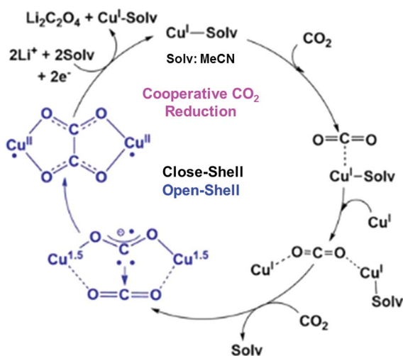
Scheme 2 Proposed catalytic cycle for one-electron reduction of CO 2 to oxalate with a copper(I) complex. Reprinted with permission from ref. 79. Copyright 2017, American Chemical Society.
