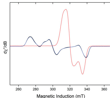
Fig. 7 Reversible binding of \text{H}_2 by [\mathbf{1}]^+[\text{BAR}_4^{\text{F}}]^- in the solid-state: CW X-band ESR spectra of powdered [\mathbf{1}]^+[\text{BAR}_4^{\text{F}}]^- under Ar (black), followed by evacuation and subsequent admission of \text{H}_2 (1 bar, [\mathbf{1}\cdot\text{H}_2]^+[\text{BAR}_4^{\text{F}}]^- , pink), and sequential evacuation to 10^{-3} mbar and backfill with Ar (blue). All spectra recorded at 40 K.
