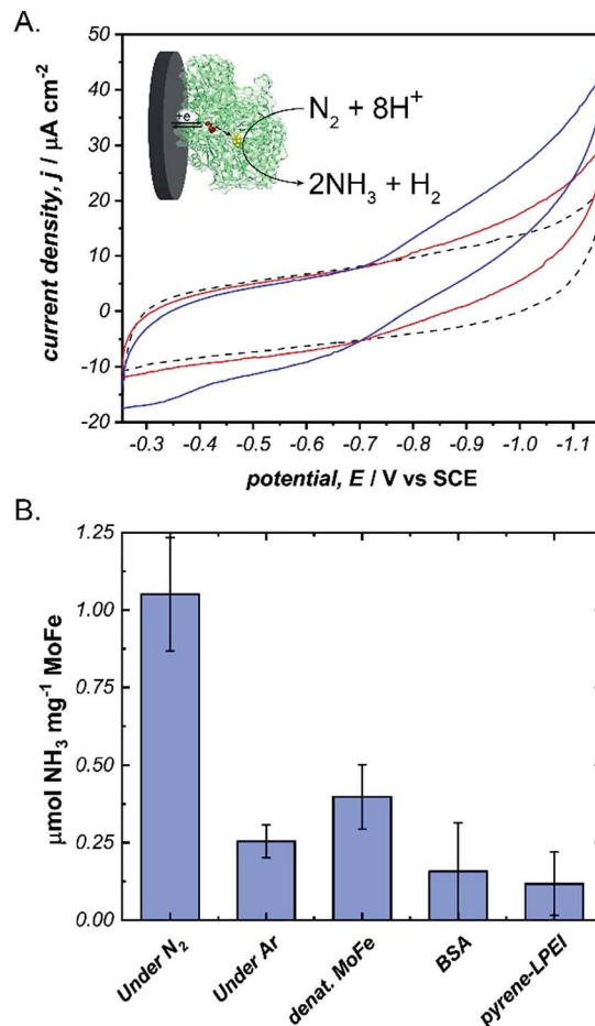
Fig. 4 (A) Cyclic voltammograms of pyrene-LPEI films containing MoFe protein and 5 mg mL -1 MWCNT-COOH under Ar (---), and after 5 min (red), or 10 min (blue) of bubbling ultra high purity \text{N}_2 . (B) Production of \text{NH}_3 using \text{N}_2 as the only substrate after constant potential bulk electrolysis of pyrene-LPEI/MoFe films for 8 h. CVs were performed using 100 mM MOPS buffer at pH 7.0, 25 °C and a scan rate of 5 mV s -1 . Bulk electrolysis was performed using 100 mM MOPS buffer pH 7.0 at -1.1 V vs. SCE and 25 °C. Error bars represent one standard deviation, where n = 3 .
