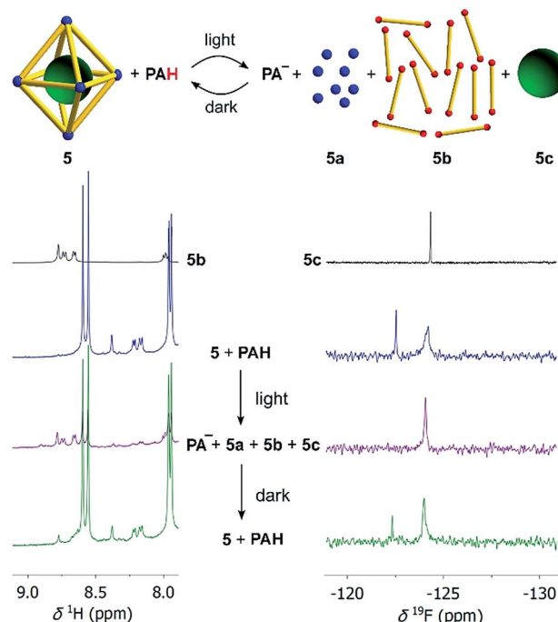
Scheme 4 Irradiation of a mixture of cage 5 ( 10\ \mu\text{M} ), NaCl ( 60\ \mu\text{M} ), and the photoacid PAH (8 equiv. with respect to each bipyridyl ligand) in \text{CD}_3\text{CN}/\text{D}_2\text{O} (8 : 2) by violet light results in disassembly of the cage and liberation of the [\text{B}(p\text{-C}_6\text{H}_4\text{F})_4]^- guest (green ball) as evidenced by the ^1\text{H} NMR (left) and ^{19}\text{F} NMR spectra (right). Details about the bridging ligand (yellow) are given in the ESI.†
