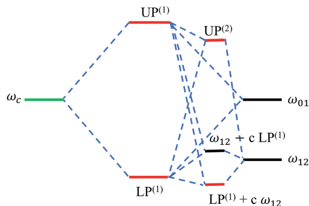
Fig. 10 Energy level hybridization diagram including the photonic ( \omega_c ) and vibrational transitions ( \omega_{01}, \omega_{12} ) involved in the formation of linear [LP^{(1)}, UP^{(1)}] and (effective) transient vibrational polaritons [UP^{(2)}, LP^{(1)} + c\omega_{12}] . 135 Note the significant interaction between the linear LP mode and the 1 \rightarrow 2 excitations (represented by the coefficient c ) arising from the incoherent population of vibrational modes induced by a pump after sufficiently long probe-delay times.
