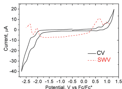
Fig. 6 Cyclic (CV) and square wave (SWV) voltammograms of 1 (1 mM) in THF (internal standard Fc/Fc*, v = 0.1 V s -1 ).
