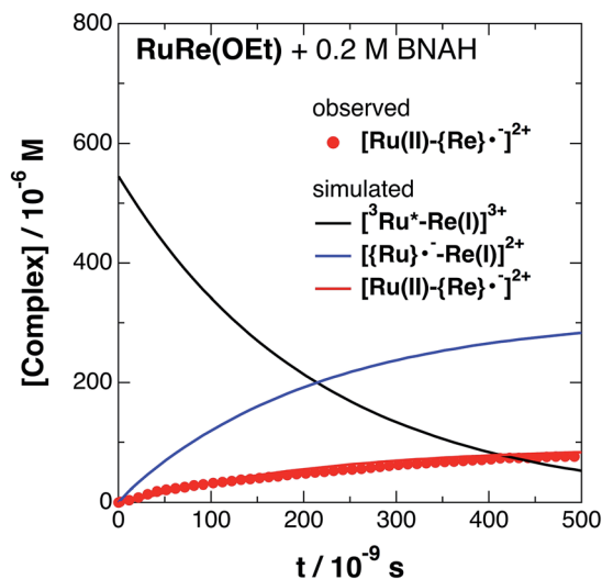
Fig. 4 Time profile of [\text{Ru(II)}-(\text{Re})^{\bullet-}]^{2+} (●) in the TRIR measurement of \text{RuRe(OEt)} in the presence of 0.2 M BNAH in an argon-saturated \text{CH}_3\text{CN/TEOA} (5 : 1 v/v) solution after 532 nm excitation. The kinetic simulation results for [\text{}^3\text{Ru}^*-\text{Re(I)}]^{3+} , [\{\text{Ru}\}^{\bullet-}-\text{Re(I)}]^{2+} , and [\text{Ru(II)}-(\text{Re})^{\bullet-}]^{2+} are also shown (solid lines).
