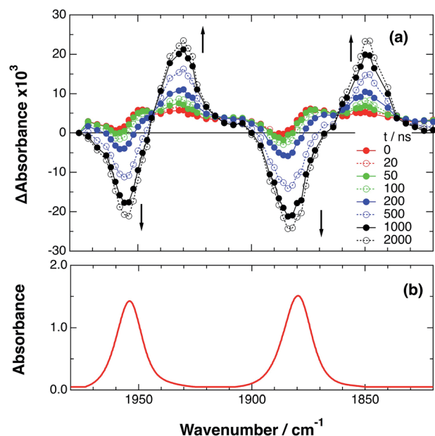
Fig. 3 (a) TRIR spectra (ns-system) recorded after 532 nm excitation of RuRe(OEt) (2 mM) in argon-saturated \text{CH}_3\text{CN}/\text{TEOA} (5 : 1 v/v) containing 0.2 M BNAH. (b) FT-IR spectrum of RuRe(OEt) in \text{CH}_3\text{CN} .
