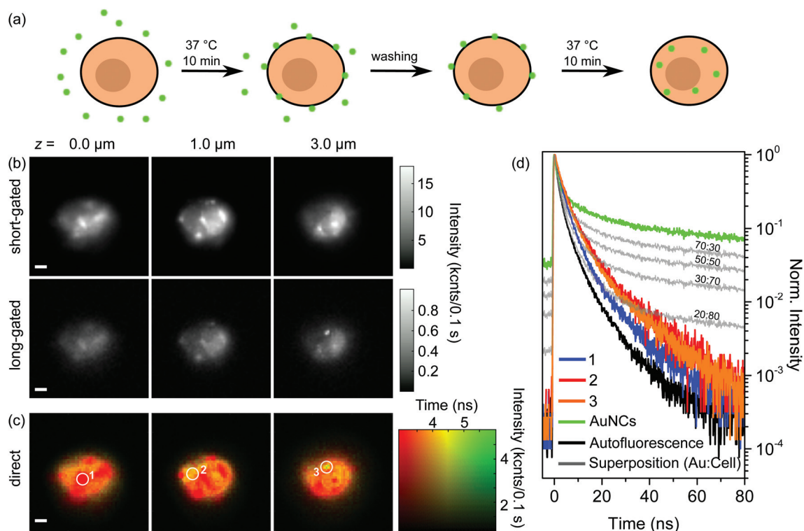
Fig. 3 (a) Sketches of the incubation process of BaF3 cells with aptamer-AuNCs. BaF3 cells were incubated for 10 min at 37 ^{\circ}\text{C} in a 4.7 nM aptamer-AuNC solution, washed three times to remove any excess of AuNCs, and then again incubated for 10 min at 37 ^{\circ}\text{C} without any addition of aptamer-AuNCs. (b) Gated and (c) direct FLIM images of two times incubated BaF3 cell aptamer-AuNCs at axial z = 0.0, 1.0, and 3.0 \mu\text{m} . (d) Fluorescence decay curves corresponding to the encircled areas in (c) (1–3, orange, red, blue) compared to decay curves (grey) calculated by superimposing the autofluorescence curve (black) and fluorescence curve of aptamer-AuNCs (green) with adjusted weighting ratios. Scale bar 2 \mu\text{m} .
