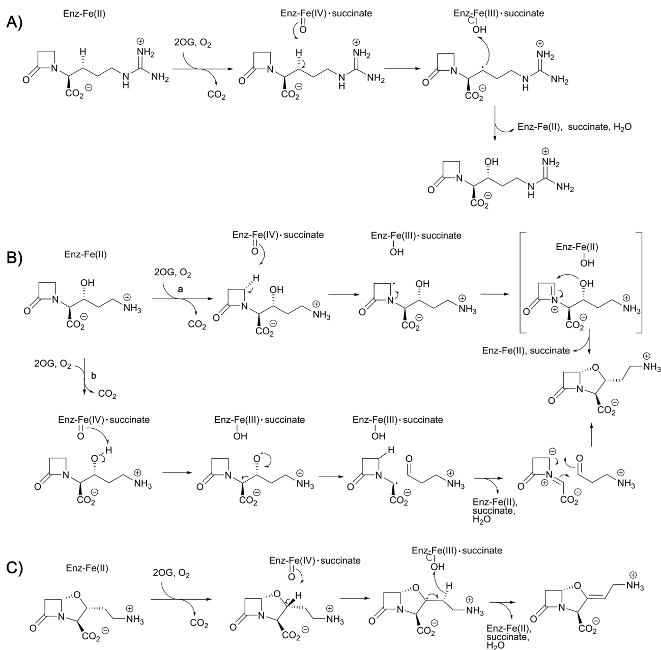
Fig. 10 Proposed outline mechanisms for the three different reactions of clavaminic acid synthase (CAS). (A) Stereoselective hydroxylation of deoxyguanidino-proclavaminc acid – a typical reaction for the 2OG oxygenases; (B) two possible mechanisms (a and b) for the oxidative cyclisation of proclavaminc acid; and (C) the desaturation of dihydroclavaminc acid.
