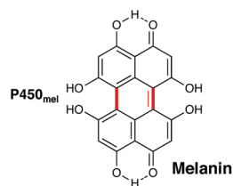
Fig. 14 Structure of melanin, the biosynthesis of which involves P450 mel in the oxidative dimerization of two 1,3,6,8-tetrahydronaphthalene subunits. The bonds introduced through P450-catalysed dimerisation are indicated in red.
