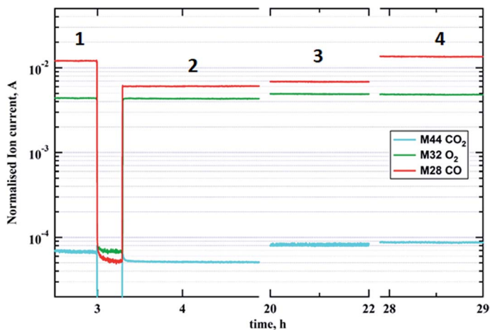
Fig. 6 MS data showing production of CO 2 during CO oxidation at 573 K over the model planar Au/SiO 2 -Si catalyst. Steps 1 and 4 correspond to a CO : O 2 ratio of 2 : 1 without and with the catalyst; steps 2 and 3 match a CO : O 2 ratio of 1 : 1 without and with catalyst, respectively.
