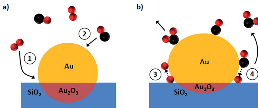
Fig. 7 Structural transformations in Au on a SiO 2 /Si(111) support during CO oxidation as revealed by operando GISAXS/GIXD. (a) Before the reaction (inert gas atmosphere) supported gold nanoparticle represents a bimodal sphere with gold oxide at the gold-substrate interface; (b) during the reaction the gold reduction takes place with the partial removal of the oxide layer as a result the submergence depth decreases whilst the particle flattens to maximise its contact perimeter.
