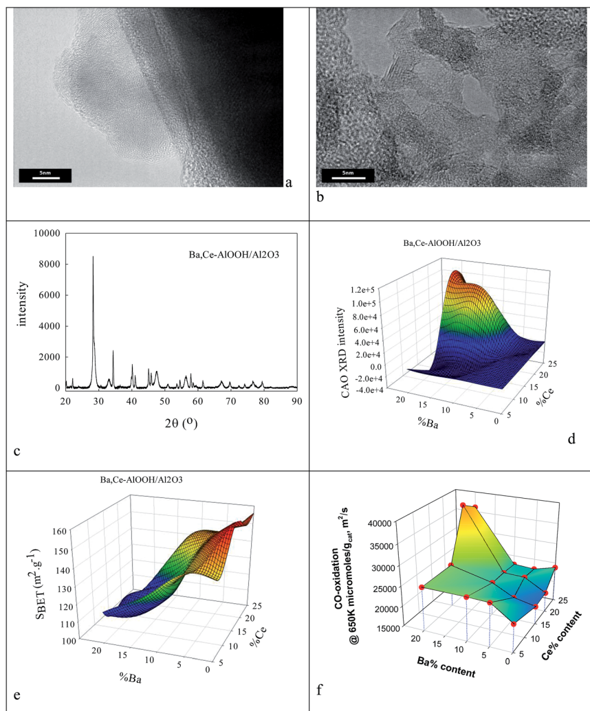
Fig. 4 Effect of Ba,Ce insertions at increasing levels into AlOOH/Al 2 O 3 after calcination at 1223 K. HRTEM (a, b), XRD structure (c) and CAO level (d), surface area (e) and CO oxidation rate at 650 K in a stoichiometric reactant stream ( R = 1.13 ).
