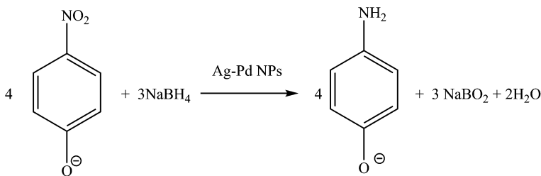
Fig. 15 Reduction of 4-nitrophenol to 4-aminophenol, \text{NaBH}_4 in excess. Conditions: 3.3 \times 10^{-5} M 4-NP and 6.6 \times 10^{-2} M \text{NaBH}_4 at room temperature.
