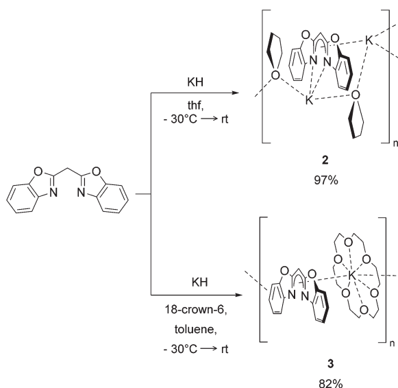
Scheme 2 Syntheses of [[\{(\text{NCOC}_6\text{H}_4)_2\text{CH}\}\text{K}(\text{thf})]_n ( 2 ) and [[\{(\text{NCOC}_6\text{H}_4)_2\text{CH}\}\text{K}(18\text{-crown-6})]_n ( 3 ) by deprotonation with KH.
