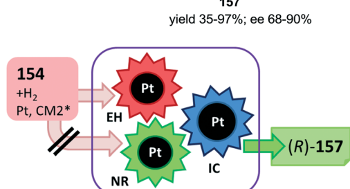
Scheme 46 Cascade EH, NR and IC of 2-nitrophenylpyruvates over chirally modified supported Pt catalyst. 203,204
