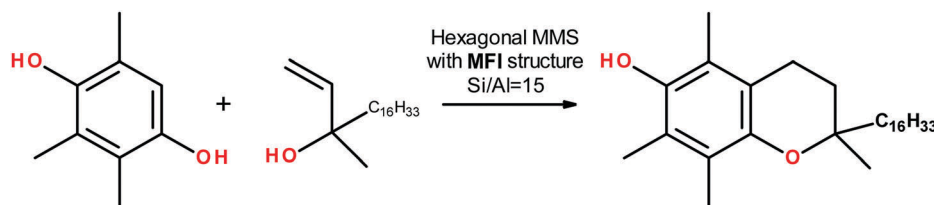
Scheme 3 Annulation of trimethylhydroquinone with isophitol yielding vitamin E.
