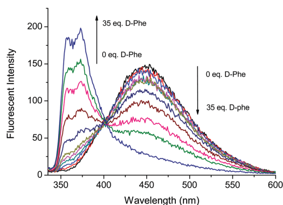
Fig. 3 Fluorescence based titrations of NI-cho1 (10 \mu M ) in CH_3CN -DMSO (95:5, v/v) with various equivalents of Boc-D-Phe.
