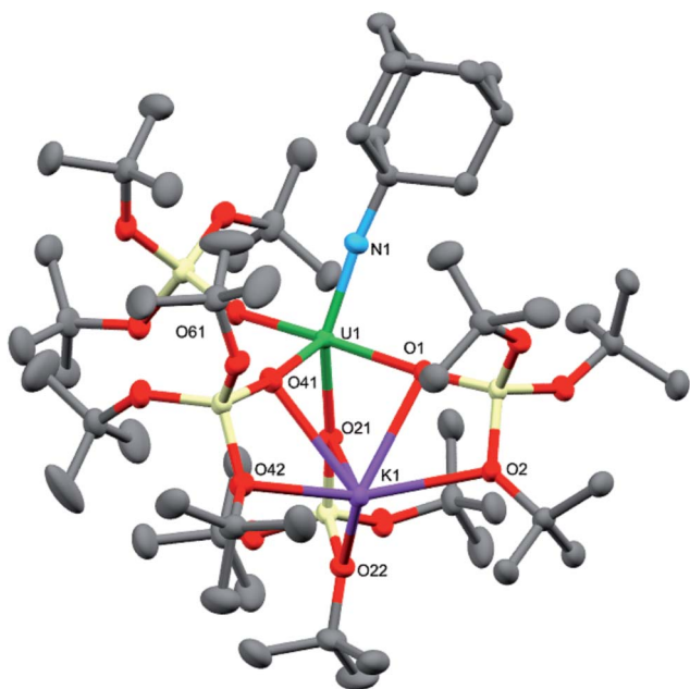
Fig. 3 Molecular structure of [U(Nad)(OSi( o Tu) 3 ] 4 K] in crystal of 4 ·tol shown with 50% probability thermal ellipsoids. Hydrogen atoms and lattice solvent have been omitted for clarity. Selected bond lengths (Å): U1–N1 = 1.954(3), U1–O1 = 2.243(3), U1–O21 = 2.175(3), U1–O41 = 2.190(3), U1–O61 = 2.185(3), K1–O1 = 2.827(3), K1–O2 = 2.631(3), K1–O21 = 3.058(3), K1–O22 = 2.626(3), K1–O41 = 2.822(4), K1–O42 = 2.725(4).
