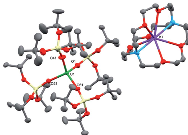
Fig. 2 Molecular structure of one of the crystallographically unique pairs of [K(2.2.2\text{-cryptand})][\text{U}\{\text{OSi}(\text{OtBu})_3\}_4] in crystals of 3 shown with 50% probability thermal ellipsoids. Hydrogen atoms have been omitted for clarity. Selected bond lengths (Å): U1–O1 = 2.223(4), U1–O21 = 2.193(4), U1–O41 = 2.211(4), U1–O61 = 2.220(4).
