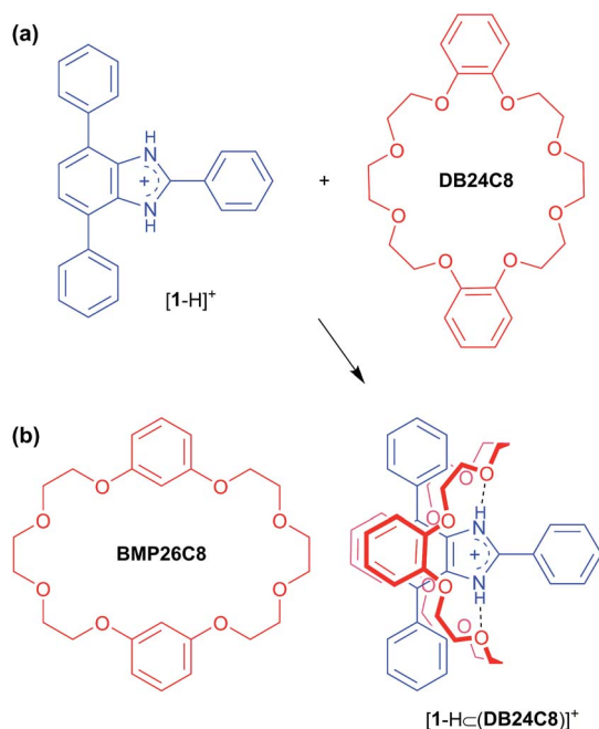
Scheme 1 (a) The [2]pseudorotaxane, [1-H⊂ DB24C8 ] + can be formed via supramolecular interactions (ion-dipole, hydrogen-bonding and \pi -stacking) between the T-shaped benzimidazolium cation, [1 – H] + and the 24-membered crown ether DB24C8 . 17,18a (b) Of relevance to this work, the crown ether BMP26C8 can also form a similar [2]pseudorotaxane, [1-H⊂ BMP26C8 ] + with [1 – H] + . 18b
