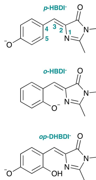
Fig. 1 Structures of the model GFP chromophores employed in this work.
