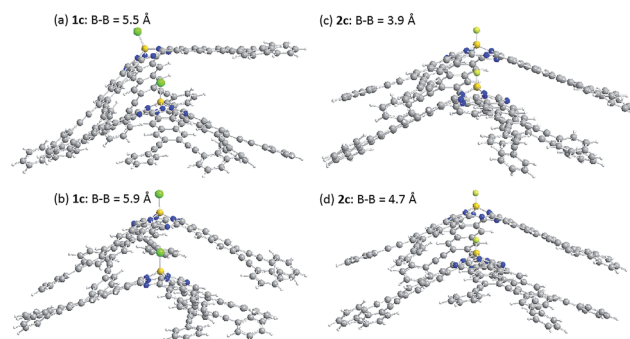
Fig. 10 Optimized structures of dimeric subnaphthalocyanines 1c and 2c . (a) 1c , B–B distance of 5.5 Å, (b) 1c , B–B distance of 5.9 Å, (c) 2c , B–B distance of 3.9 Å, and (d) 2c , B–B distance of 4.7 Å.
