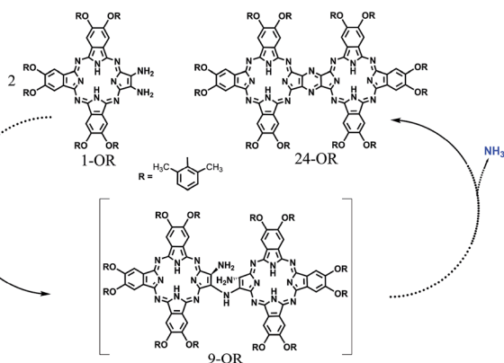
Scheme 3 Schematic of the reaction pathway of the formation of 24-OR with 1-OR as the starting reagent though 9-OR together with the formation of ammonia.
