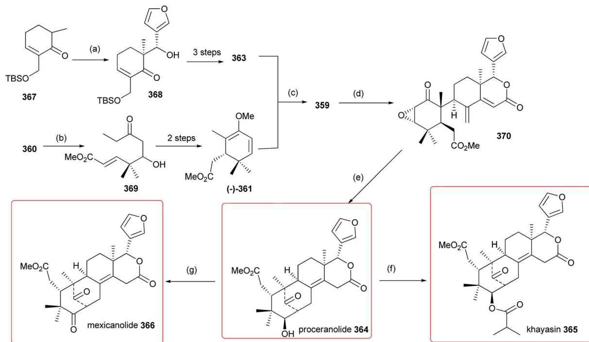
Scheme 2 Reagents and conditions: (a) (i) KHMDS, THF, -78\text{ }^{\circ}\text{C} , then (–)-DIP-Cl, (ii) 3-furylaldehyde, 33–44% yield, 80–90% ee; (b) (+)-DIP-Cl, DIPEA, 2-butanone, Et 2 O, -78\text{ }^{\circ}\text{C} , then -105\text{ }^{\circ}\text{C} to -30\text{ }^{\circ}\text{C} , 16 h, 47% yield, 92.5% ee; (c) TsOH, xylenes, 180\text{ }^{\circ}\text{C} , 4 h; (d) 30% H 2 O 2 , K 2 CO 3 , MeOH, 0\text{ }^{\circ}\text{C} to r.t., 12 h, 75%; (e) Al/Hg, EtOH/THF/H 2 O/NaHCO 3 , r.t., 1 h, 30%; (f) isobutyric acid, EDCl, DMAP, CH 2 Cl 2 , 0\text{ }^{\circ}\text{C} to r.t., 4 h, 71%; (g) K 2 Cr 2 O 7 /H 2 SO 4 , Me 2 CO, r.t., 15 min, 68%.
