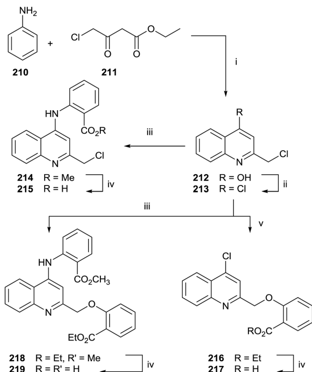
Scheme 37 Reagents and conditions: (i) PPA, 130^\circ\text{C} , 1 h. (ii) \text{POCl}_3 , 100^\circ\text{C} , 3 h. (iii) Methyl 2-aminobenzoate, \text{C}_2\text{H}_5\text{OH} , conc. \text{HCl} , 5 h. (iv) \text{THF}/\text{MeOH} , \text{LiOH} , 3 h. (v) Ethyl-2-hydroxybenzoate, \text{K}_2\text{CO}_3 , \text{CH}_3\text{CN} , 90^\circ\text{C} , 5 h.
