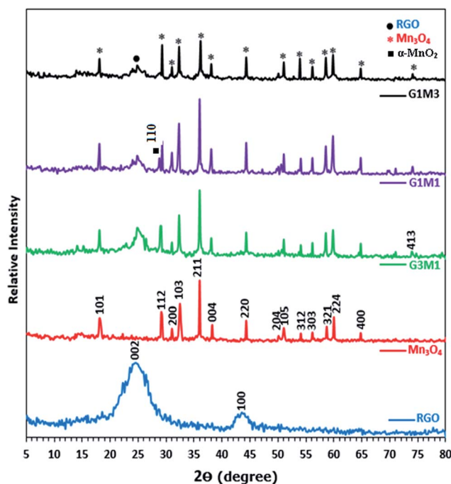
Fig. 1 XRD patterns of RGO, \text{Mn}_3\text{O}_4 , G3M1, G1M1 and G1M3.
