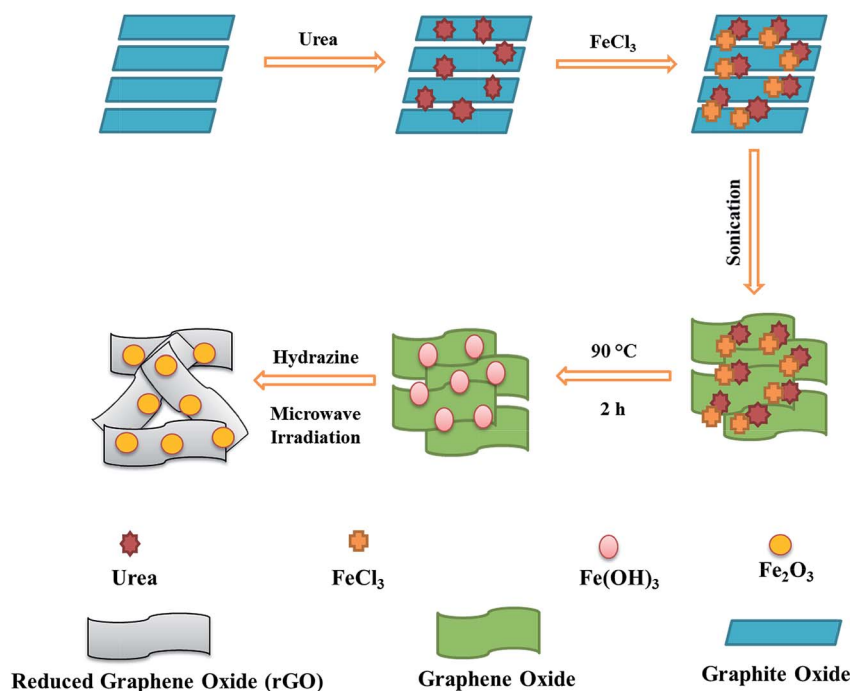
Scheme 1 Schematic of fabrication of rGO- \text{Fe}_2\text{O}_3 composite.
