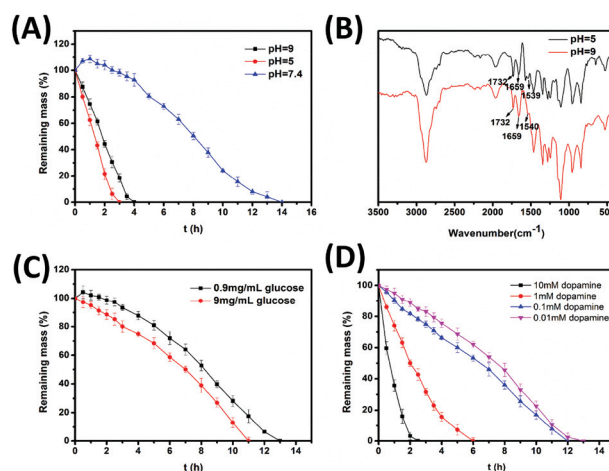
Fig. 3 The degradation behavior of hydrogels at 37\text{ }^{\circ}\text{C} : (A) pH responsive degradation of hydrogels; (B) mechanisms of degradation at different pH values; (C) glucose responsive degradation of hydrogels; (D) dopamine responsive degradation of hydrogels.
