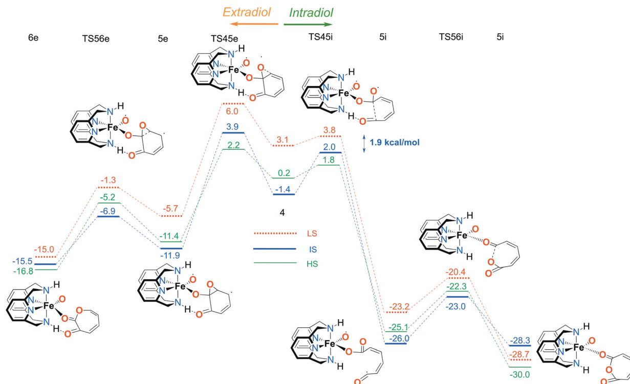
Fig. 5 Calculated reaction profile for the second part of the catalytic mechanism with the LN 4 H 2 ligand, branching to the extradiol (left) and intradiol (right) pathways. Electronic energies (kcal mol -1 ), obtained using the S12g/TZ2P level of theory, are given relative to reactants.
