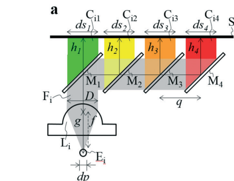
Fig. 1 Diagram of an ultra-small four-color ( C_{ij} ) detection system for a four-emission-point array ( E_i ), where i = 1 to 4 (emission-point number) and j = 1 to 4 (color number), using a four-lens array ( L_j ), a four-dichroic-mirror array ( M_j ), and an image sensor (S); dp: diameter of E_i ; f : focal length of L_j ; D : effective diameter of L_j ; g : emission-point distance; h_j : sensor distance for C_{ij} ; p : intervals between emission points ( E_i ) and between lenses ( L_j ); q : interval between mirrors ( M_j ); and ds_j : diameter of image of C_{ij} . (a) Cross-sectional view perpendicular to E_i and (b) planar view parallel to E_i . (c) Optimal conditions for an ultra-small detection system with high sensitivity and low crosstalk, where dp = 0.05 mm, p = 1 mm, and p < q .
