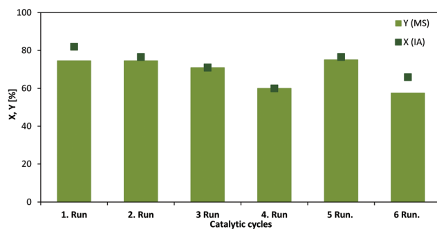
Fig. 5 Chemo-catalytic batch hydrogenation of IA over a Ru/C catalyst including recycling: 100 mg Ru/C in pure IA solution (0.61 mol L -1 , 9.1 mmol, 1.187 g). Reaction conditions: 1 h, 70 °C, 10 bar of H 2 , 15 mL water, 500 rpm stirring speed.
