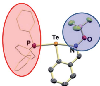
Fig. 13 N–Te⋯P chalcogen bond. Strong chalcogen bonding capability of Te is activated by coordination of N-oxide, and further enhanced by Lewis acid coordination of the \text{BF}_3 group to the oxygen (blue circle). Phosphine ( \text{PPh}_3 , red ellipse) serves as the (Lewis basic) chalcogen bond acceptor. Adapted from DOI: 10.1039/c7fd00075h with permission from The Royal Society of Chemistry.
