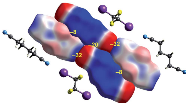
Fig. 9 1,4-Dicyanobutane:1,2-diiodo-1,1,2,2-tetrafluoroethane co-crystal (EBIHII): ESP mapped on Hirshfeld surfaces for a cluster of molecules in the crystal. Colour mapping and range for ESP as for Fig. 1, and the electrostatic interaction energies ( \text{kJ mol}^{-1} ) for nearest neighbour pairs of molecules are indicated in yellow.
