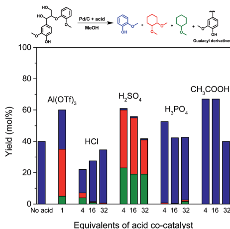
Fig. 4 Reactions of guaiacylglycerol-β-guaiacyl ether (GG) in methanol over Pd/C and/or different acid co-catalysts at 160 °C for 2 h in 30 bar H 2 .
