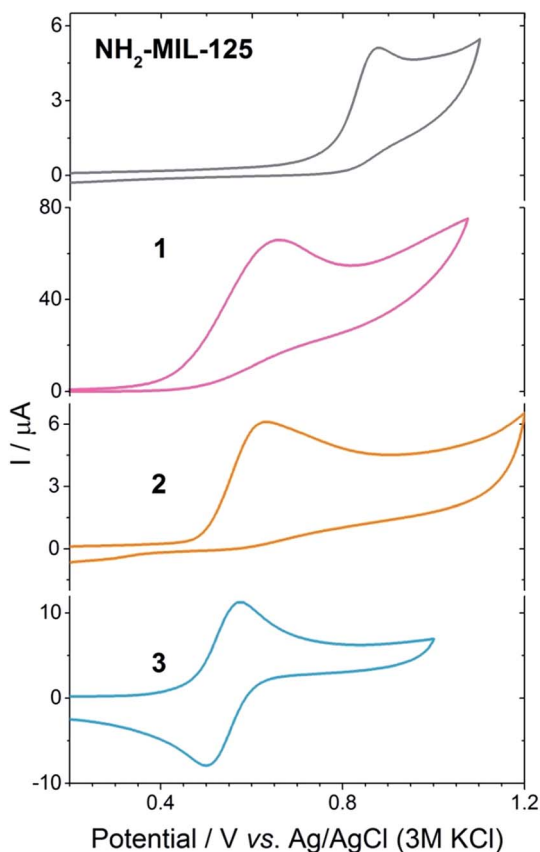
Fig. 4 Cyclic voltammetry at 50 \text{ mV s}^{-1} of \text{NH}_2\text{-MIL-125(Ti)} , 1 , 2 (phosphate buffer, pH 7) and 3 (0.1 M \text{LiClO}_4 ) in water as it is the only medium that allowed for electrochemical measurements of the MOF.
