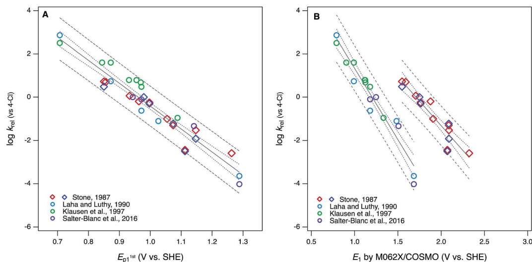
Fig. 5 Correlations of rate constants for oxidation by manganese oxides ( k_{rel} ) and oxidation potentials of phenols and anilines: (A) \log k_{rel} from compiled sources (Table S1 † ) vs. E_{p1}^{1st} from this study (Tables S4 and S5 † ); (B) \log k_{rel} vs. E_1 without calibration, from this study (Tables S6 and S7 † ). Diamonds represent phenols and circles represent anilines.
