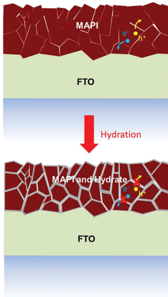
Fig. 11 Microscopic degradation model of MAPI thin films under partial hydration. Reproduced from ref. 94, Copyright 2015 American Chemical Society.
