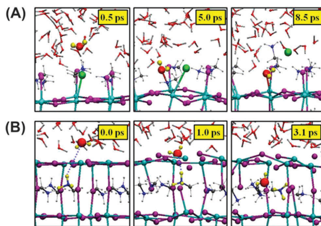
Fig. 12 (A) Nucleophilic substitution of a surface iodide atom by a water molecule in the MAI-terminated \text{MAPbI}_3 slab. (B) Incorporation of a water molecule to the \text{PbI}_2 -terminated slab. Adapted from ref. 110, Copyright 2015 American Chemical Society.
