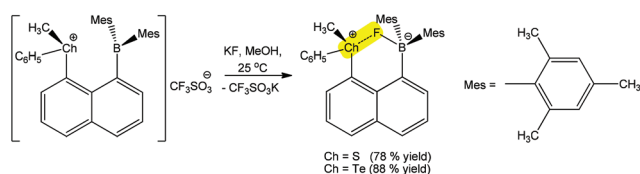
Scheme 27 Positive charge assisted chalcogen bonding in the recognition of \text{F}^- by (\text{R})\text{-}[(\text{8-(dimesitylboryl)naphthalen-1-yl)(methyl)(phenyl)chalconium}]^+\text{CF}_3\text{SO}_3^- trifluoromethanesulfonates. 181
