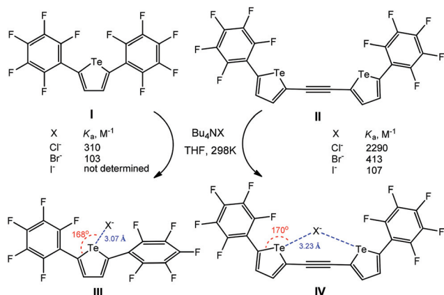
Scheme 28 Negative charge assisted chalcogen bonding in the recognition of \text{X}^- by perfluoroaryl-substituted tellurophenes. 113
