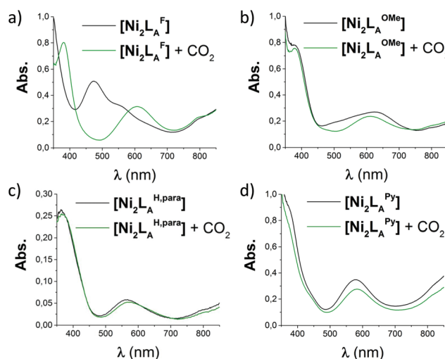
Fig. 2 UV-vis spectra (MeCN/MeOH 4 : 1, RT) of the reaction of [\text{Ni}_2\text{L}_A^{\text{R}}](\text{Cl})(\text{ClO}_4)_3 with \text{CO}_2 : (a) [\text{Ni}_2\text{L}_A^{\text{F}}] , (b) [\text{Ni}_2\text{L}_A^{\text{OMe}}] , (c) [\text{Ni}_2\text{L}_A^{\text{H,para}}] and (d) [\text{Ni}_2\text{L}_A^{\text{Py}}] .
