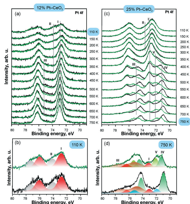
Fig. 17 Pt 4f spectra obtained from 12% Pt–CeO 2 (a and b) and 25% Pt–CeO 2 (c and d) films prepared at 110 K on CeO 2 (111)/Cu(111) annealed at different temperatures (black) and exposed to 50 L of CO at 110 K (green); the structure of the Pt 4f spectra on as-prepared 12% Pt–CeO 2 at 110 K (b) and 25% Pt–CeO 2 films annealed to 750 K (d); the components labelled I–V arise from Pt 2+ , Pt 4+ , Cu 3p, and metallic Pt particles (IV–V), respectively. Adapted from ref. 112 with permission from the PCCP Owner Societies.
